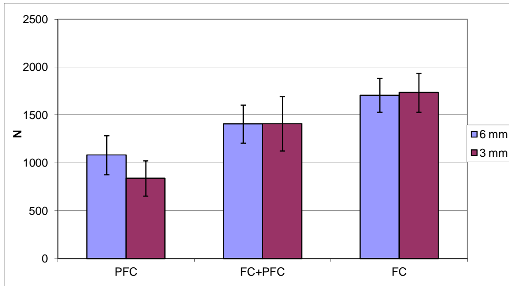
Fig. (2). Mean values of compressive load-bearing capacity of onlay restorations. N refers to Newton. PFC refers to particulate filler composite resin. FC refers to short fiber composite. FC+PFC refers to materials combination of FC substructure and covered with a 1 mm layer of PFC. Vertical lines represent standard deviations.
