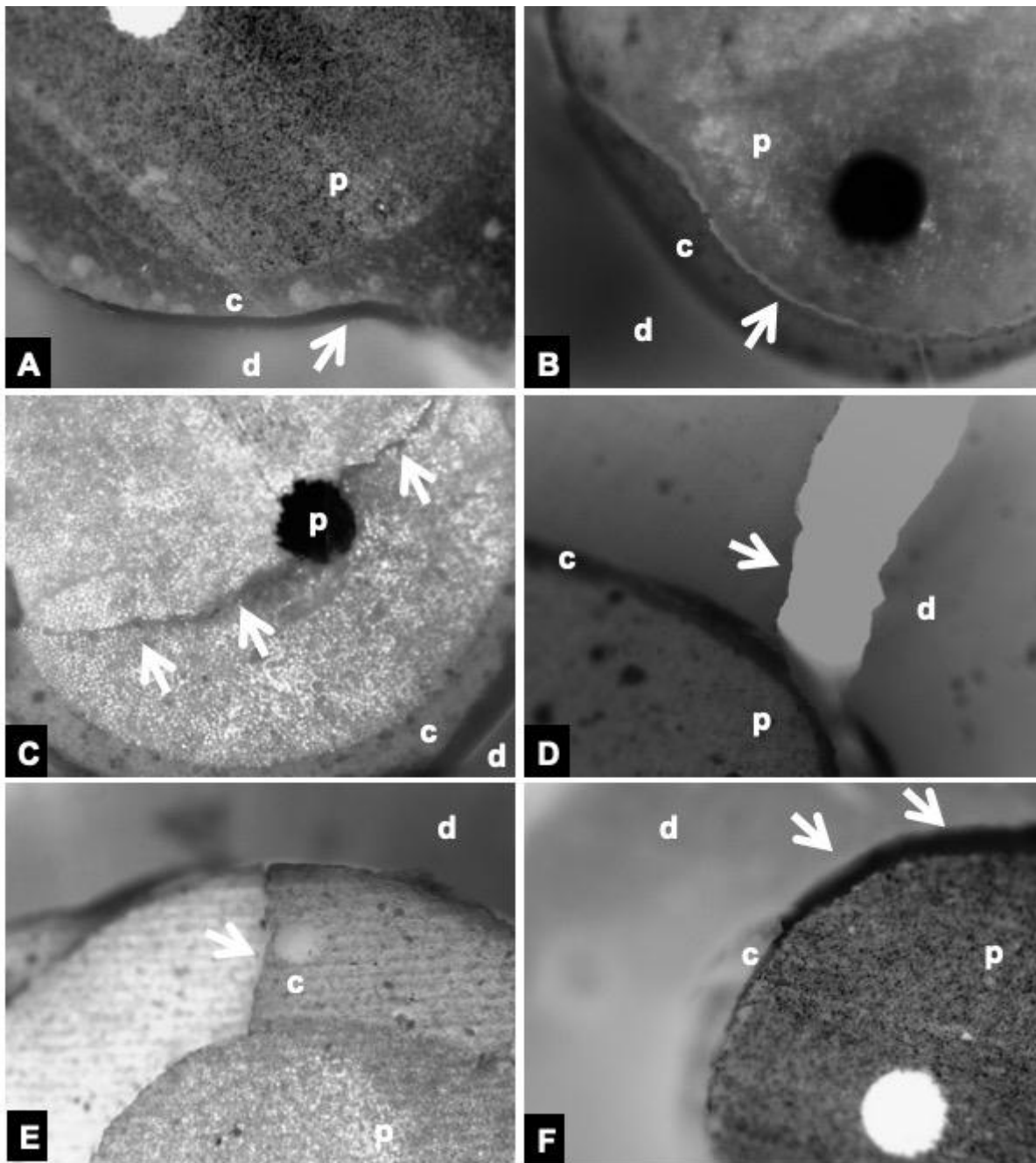
Fig. (1). Light microscopy of failure mode: (a) adhesive between resin cement and root dentin, (b) adhesive between resin cement and post, (c) cohesive in post, (d) cohesive in dentin, (e) cohesive in cement, (f) mixed, between post, resin cement and root dentin. White arrows point the failure area. d = dentin, c = resin cement, p = fiber glass post.
